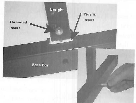
Finger Bolt is threaded into Upright from outside of Base Bar
